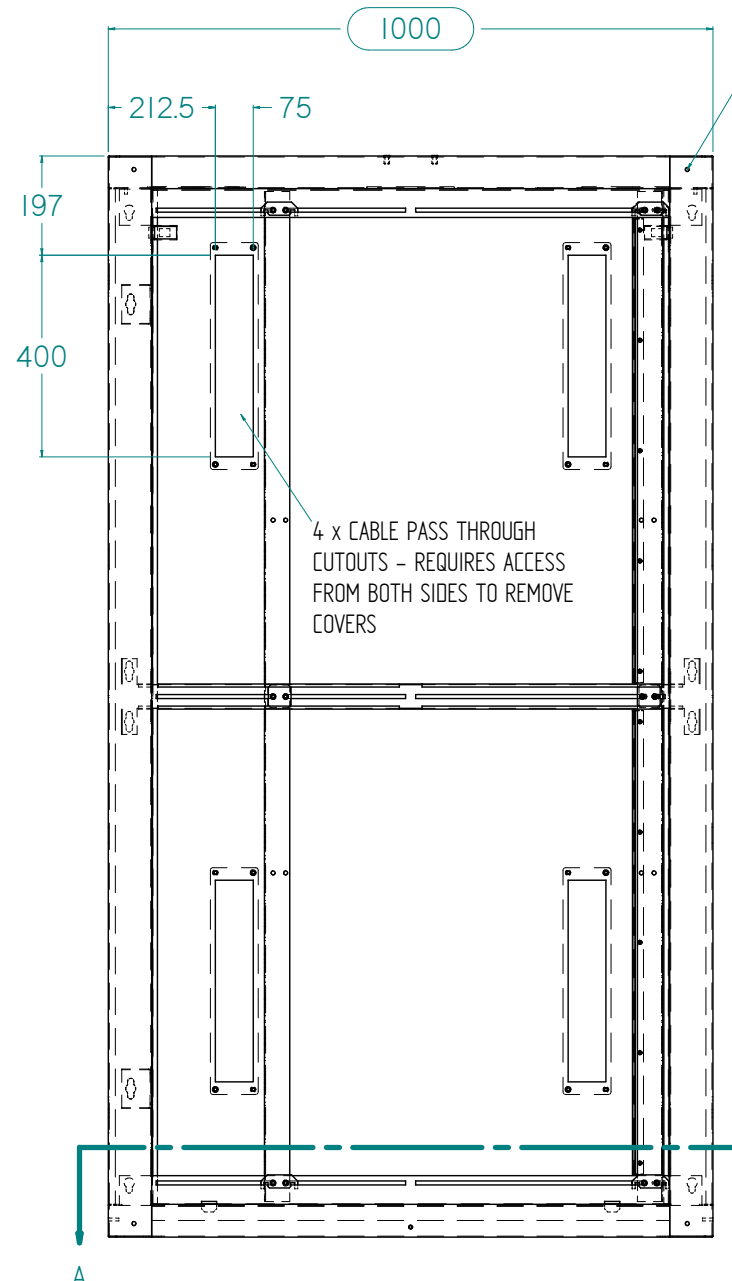
LEFT SIDE VIEW PANEL REMOVED
