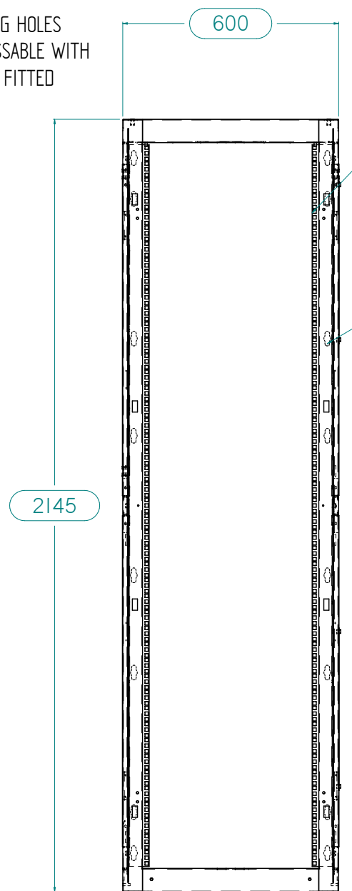
FRONT VIEW DOORS REMOVED
