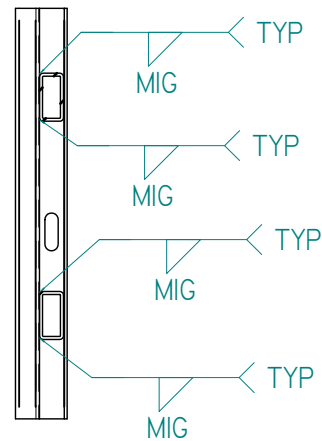
TYPICAL WELD EVERY HORIZONTAL & VERTICAL BAR SECTION B-B 1:4
