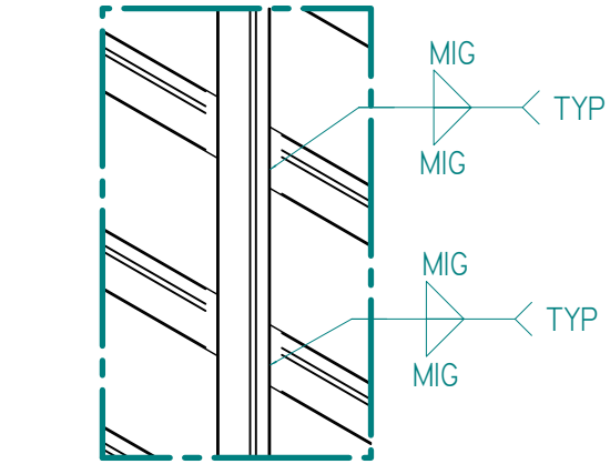
TYPICAL WELD EVERY HORIZONTAL & VERTICAL BAR DETAIL C 1:4
